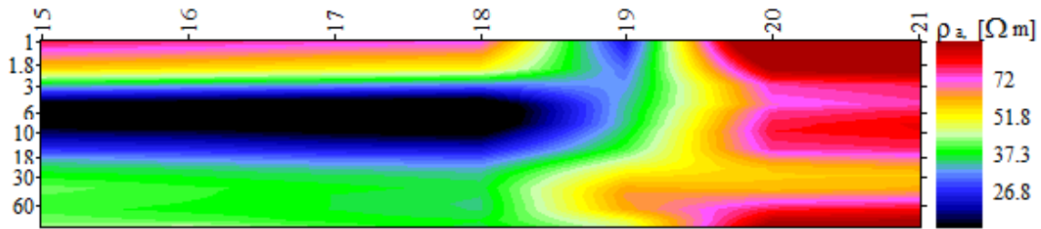
Resistivity cross-section
