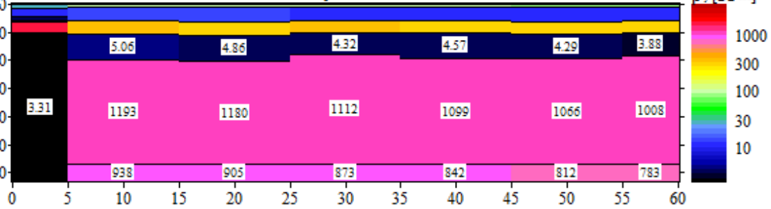
Resistivity cross-section
