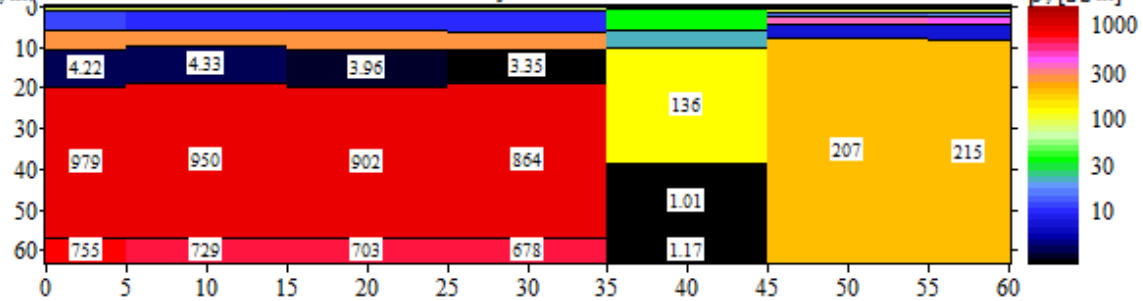
Resistivity cross-section
